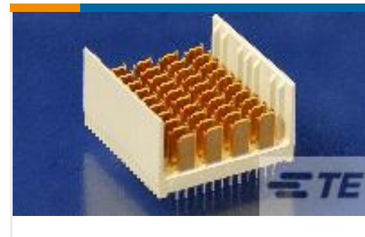
TE 产品编号6469002-1 HM-ZD 4PR HDR 80P 5.2MM
