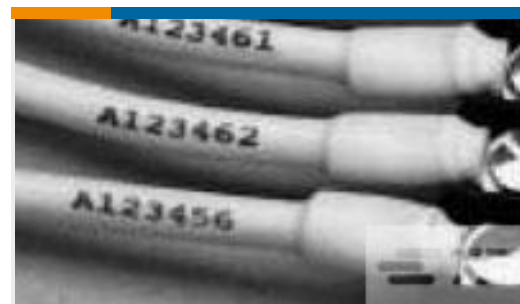
TE 产品编号EG8142-000 RNF-100-3/32-WH-85MM
