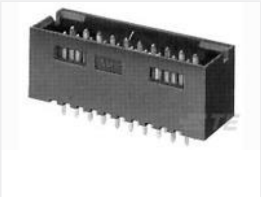
TE 产品编号6-103169-0 24 MODII HDR DRST SHRD .100CL
