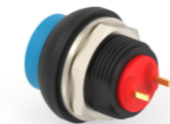
TE 产品编号2-2329328-0 PB OFF/ON HC BLU M4 TERM. IP68
