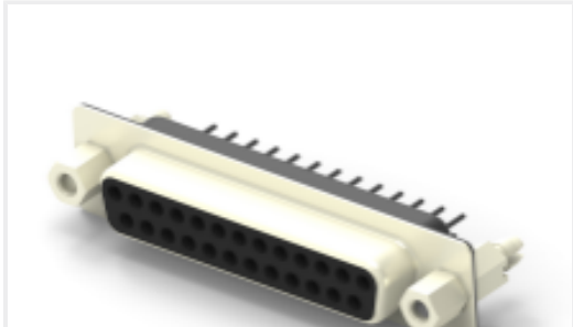
TE 产品编号2301841-2 AMPL REC HD20, VERT, 25P, B/L,4-40 S/LOC
