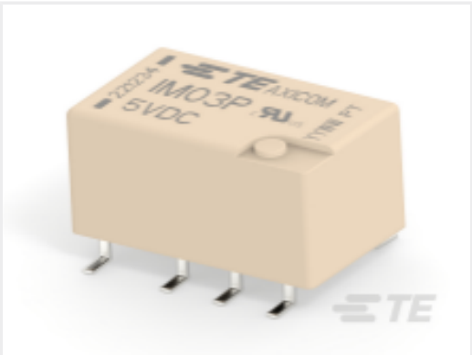
TE 产品编号 5-1462039-5 IM03PGR=IM RELAY 140mW 5V
