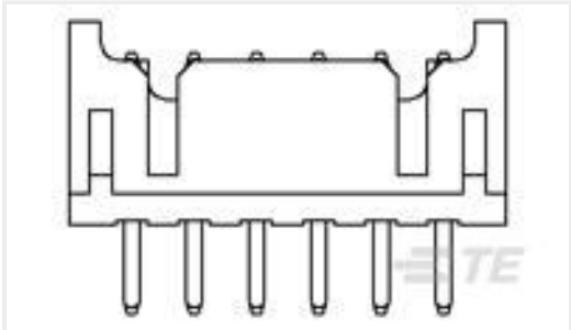
TE 产品编号 8-1470109-0 2.0MM HDR, 30 POS, DIP, soldertail 2.40
