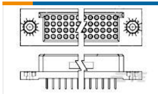
TE 产品编号533499-2 BOX II 4 ROW RECP ASSY 232 POS
