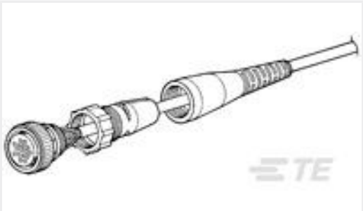
TE 产品编号207387-2 CABLE GRIP,SZ 17,CPC
