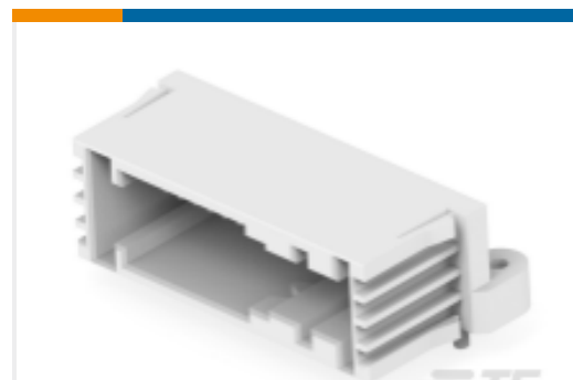
TE 产品编号2-968720-4 32pos MQS .63 header 90deg
