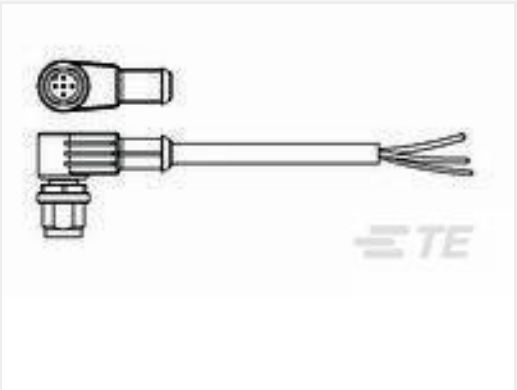
TE 产品编号2273076-3 M12 x 1.0 angled plug pigt A
