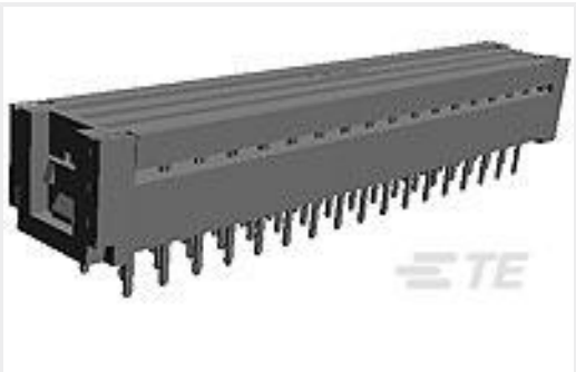
TE 产品编号1-5111595-2 060 ASSY SYS 50 PADDLEBOARD
