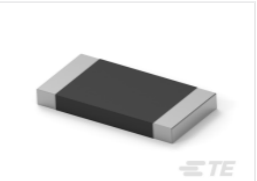
TE 产品编号3-2176421-7 TLRP 2512 2.0W R100 1% 25PPM 4K RL
