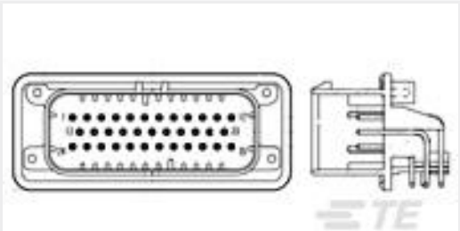
TE 产品编号1-776163-1 35POS,PIN DIA 1.3,HDR ASSY,90DEG, COD 1
