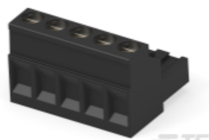
TE 产品编号 796641-5 5 POS 5.0 MM R/A PLUG, TRM BLK
