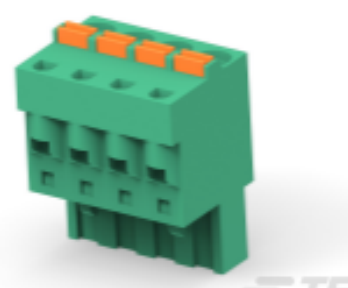
TE 产品编号 1546557-5 5P, SCREWLESS CLIP PLUG, 5.0MM
