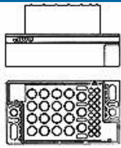
TE 产品编号 796299-1 AMPOWER HOUSING, RCPT, 35 POS
