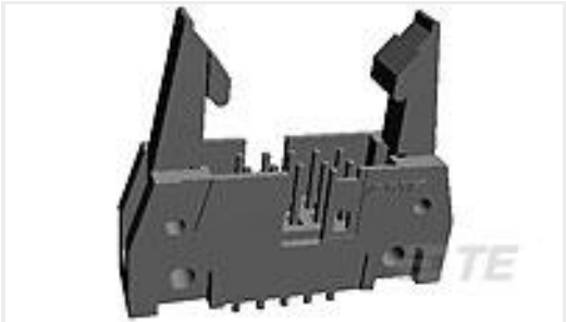
TE 产品编号5746443-8 A/L UNIV HDR 34P ACT PIN LAT
