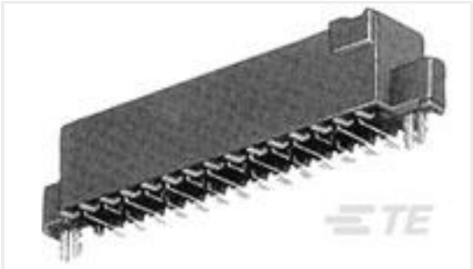
TE 产品编号5-104652-8 80 50/50 GRID DRST SFMNT RCPT
