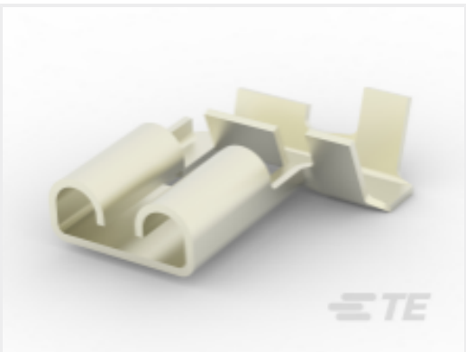
TE 产品编号2286377-1 250 FASTON,FLAG,REC.,22-18 AWG, NPST
