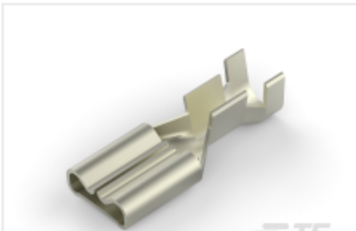
TE 产品编号2238199-3 FASTON 187 STD REC STR 18-14TPBR
