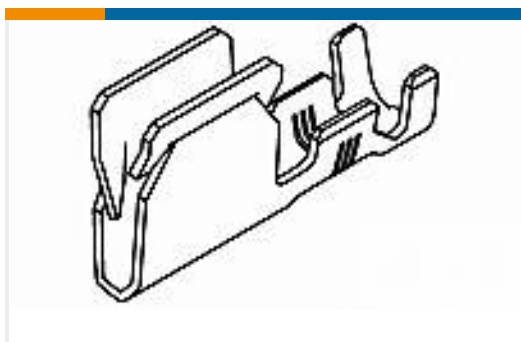
TE 产品编号63895-1 GROUND CLIP 14-18AWG ST
