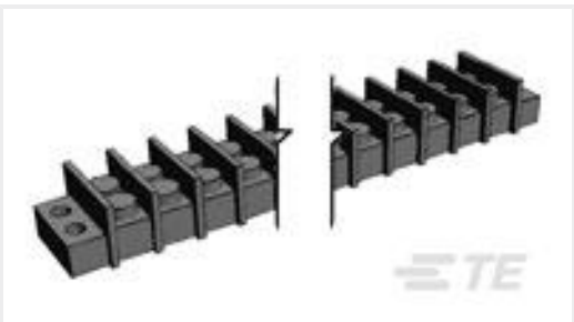
TE 产品编号5-1546306-0 7P .374" DR, Flat QC, DS Custom
