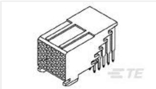
TE 产品编号5223008-1 FB-5R,ASY,030,SIG,REC,EN,3.55
