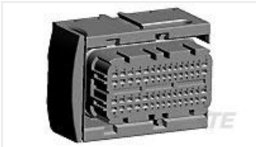
TE 产品编号2-1355123-3 CARRIER HSG 60POS,ASSY
