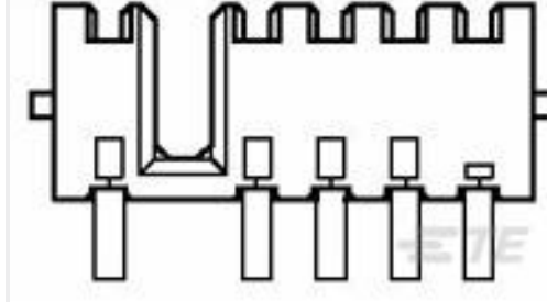
TE 产品编号1747367-1 RECEPTACLE ASSEMBLY 2.5MM PITCH BATTERY
