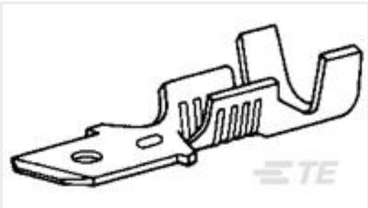
TE 产品编号62531-1 205 FASTON TAB 18-14 AWG TPBR
