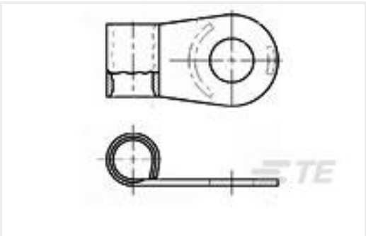
TE 产品编号322727 TERMINAL,SOLIS FLAG R 8 1/4
