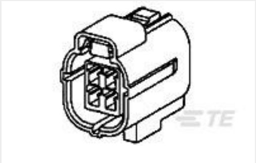
TE 产品编号CAT-AM7801-CH8172 AMPSEAL 16 Housings
