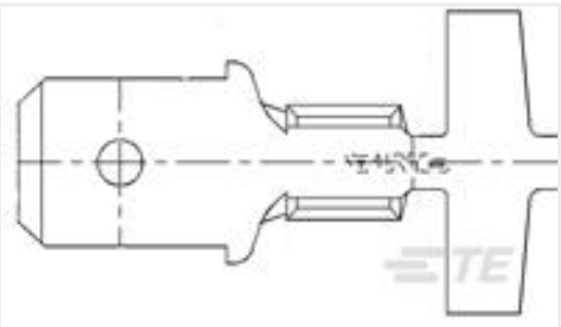
TE 产品编号61367-3 250 FASTON TAB 18-14 AWG TPBR
