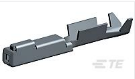
TE 产品编号1318332-1 .040 SEALED REC CONT
