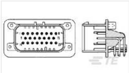
TE 产品编号1-776087-5 23POS,PIN DIA 1.3,HDR ASSY,90DEG, COD 5
