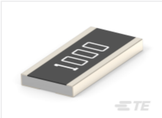
TE 产品编号8-2176566-5 3430 A3 1% 3K0 100ppm 1k RL
