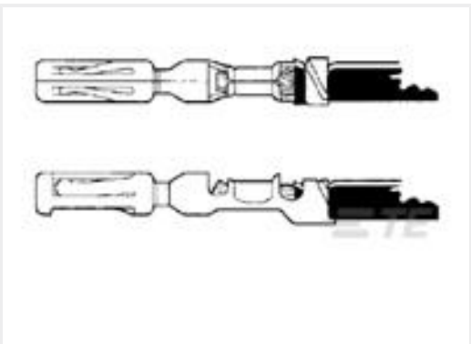
TE 产品编号770854-3 CONTACT,AMPSEAL AU L/P
