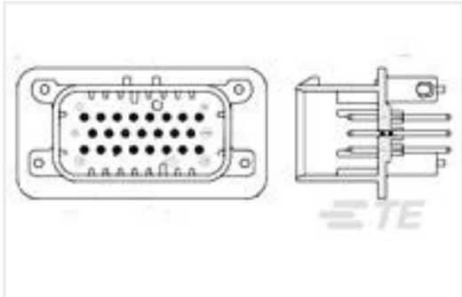
TE 产品编号776231-1 35POS,PIN DIA 1.3,HDR ASSY, 180DEG,COD 1
