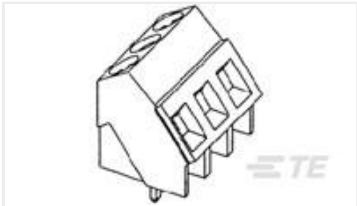
TE 产品编号282847-7 TERMI-BLOK PCB MOUNT 35 7P.5
