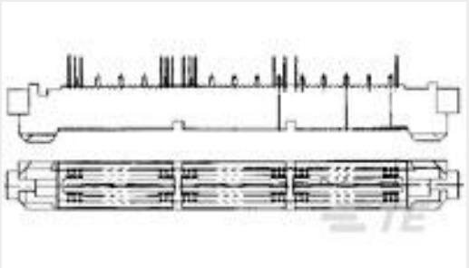
TE 产品编号 767039-1 MICTOR,RA PLUG,038,.093PCB,ASY
