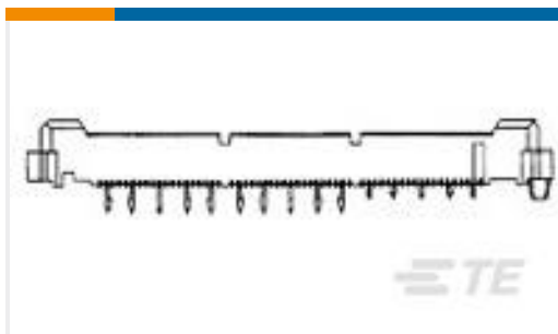
TE 产品编号 767089-6 MICTOR,R/A,RECPT,.093,228,ASY
