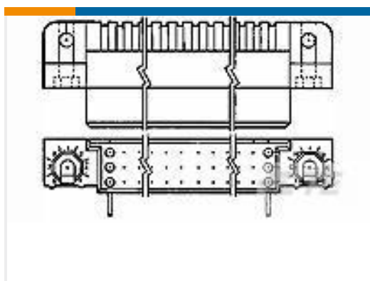
TE 产品编号532431-3 HDI RECP ASSY 3 ROW 96 POS
