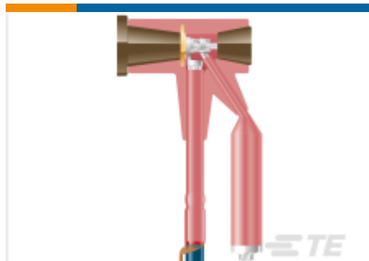
TE 产品编号555340-014 RICS Insulated T-Adapter
