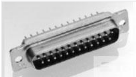
TE 产品编号204507-1 AMPLIMITE,ASY,PLUG,STD,90,4
