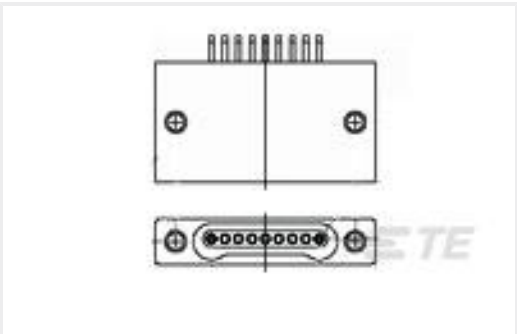
TE 产品编号1589462-9 SSL009L2HN = SMT CONN
