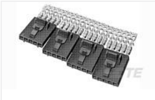
TE 产品编号103957-7 2X8 MTE RCPT SR LATCH .100CL
