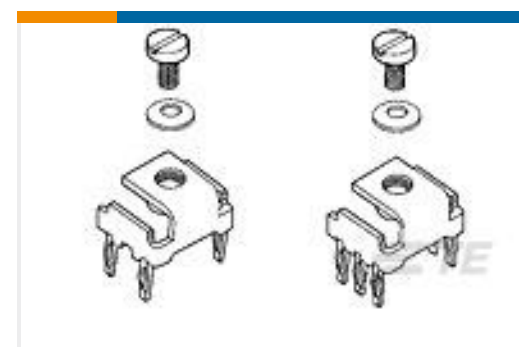
TE 产品编号5213816-1 6P POWER TAP ASSY W/M4 SCREW
