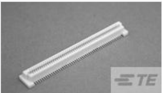
TE 产品编号5-1735480-1 0.8FH,R17H.5,040,08/Sn,TU
