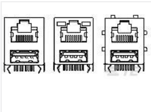
TE 产品编号5-1775855-1 RJ45 OVER USB W/ 6 PNL-GND & HTD G/F
