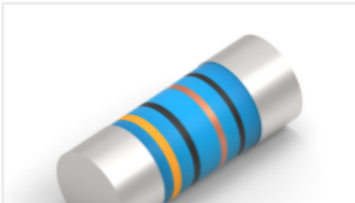
TE 产品编号2-2176315-6 MELF SMA_A 12K 0.1% 15PPM 0204 0.4W
