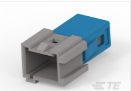
TE 产品编号284869-4 8POS MQS TAB
