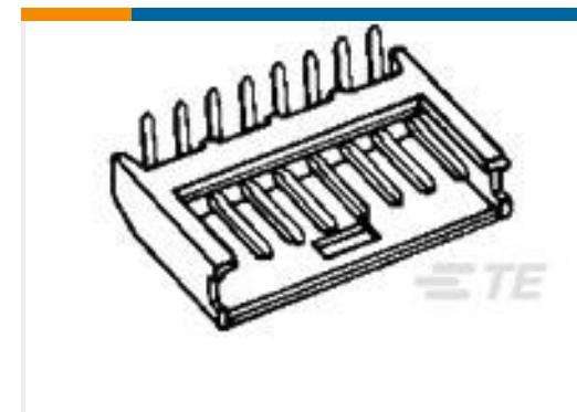
TE 产品编号280378-2 4P MODU II SHRD HDR, RT ANG, 0.38 AU
