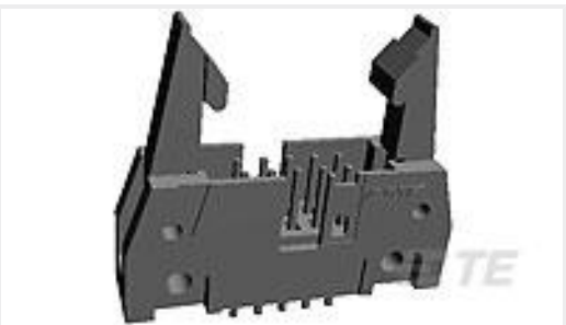
TE 产品编号5499160-4 A/L UNIV HDR 20P VERT SHT LAT
