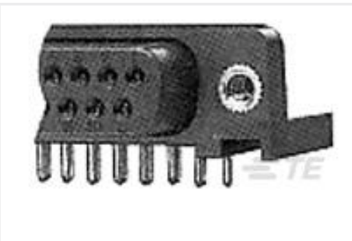
TE 产品编号5788796-1 09 HTMSFL ASSY RA 318 (IN,BL)
