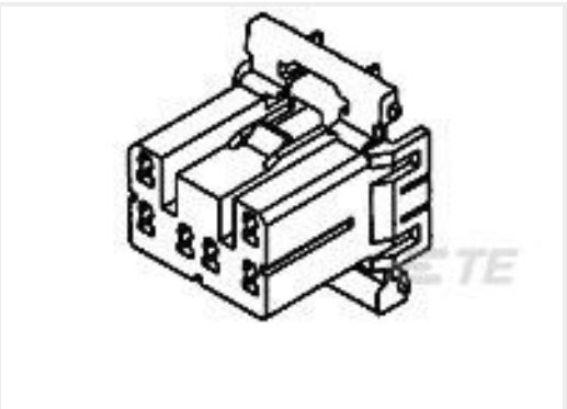
TE 产品编号368511-1 070 MLC PLUG 20P HSG
